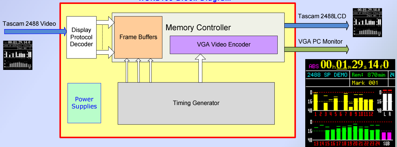
HGR2488 Block Diagram
